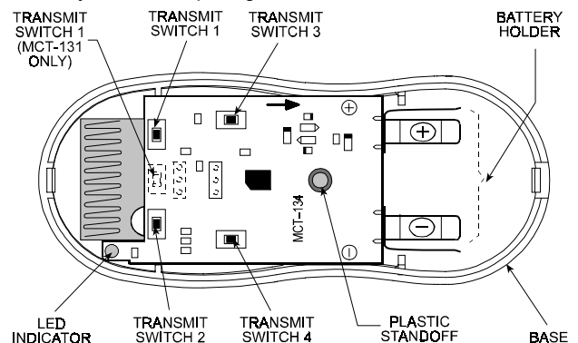
Figure 3. Component Layout
